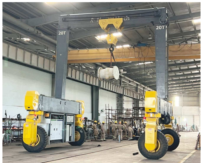
Valve parts handling (indoor application)
