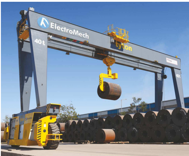
Steel coil handling
